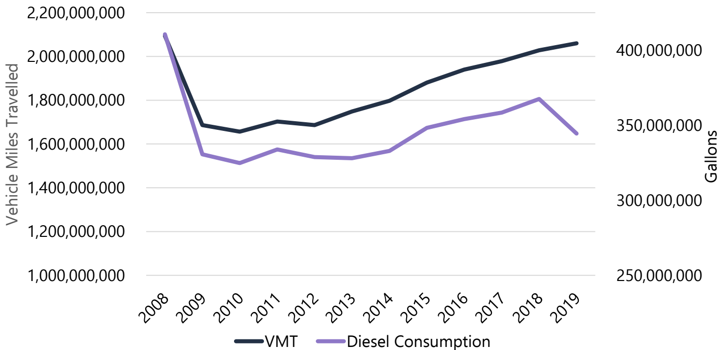
Figure 4: Oregon VMT and Fuel Consumption of Heavy Trucks (Greater than 34,001 Pounds) 16
