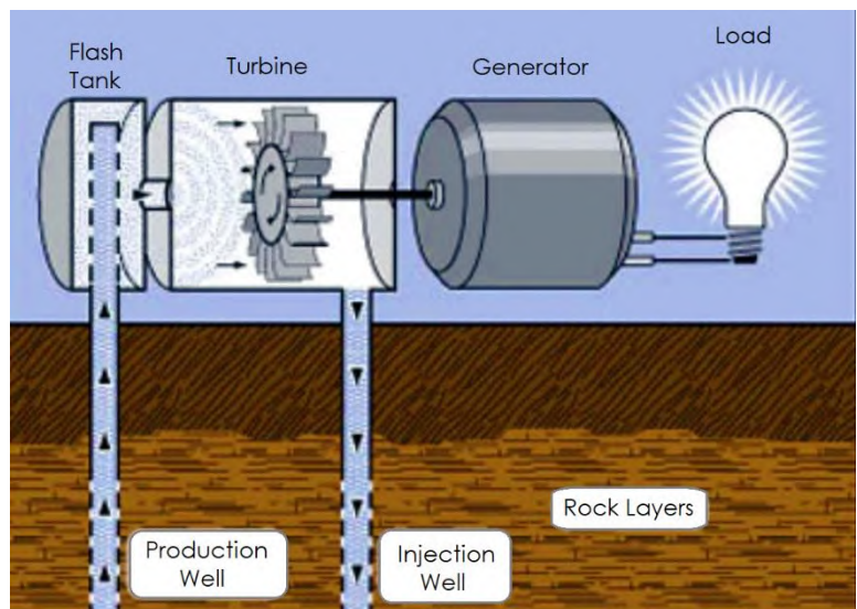
Figure 1: Flash Steam Power Plant 8
