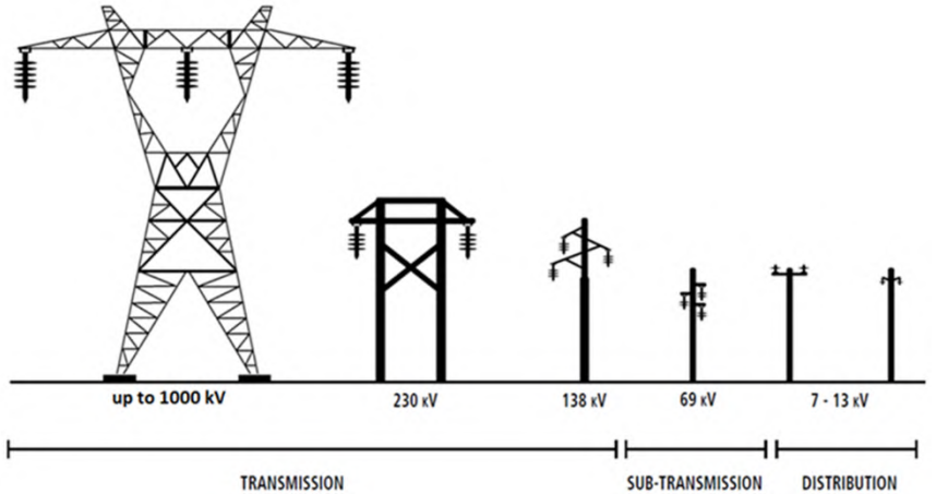
Figure 1: Typical Sizes of Transmission and Distribution Systems
