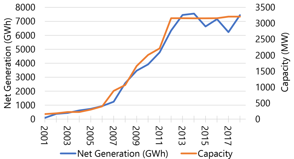
Figure 2: Wind Net Generation and Capacity in Oregon by Year
