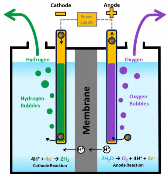
Figure 1: Electrolyzer Illustration 4
